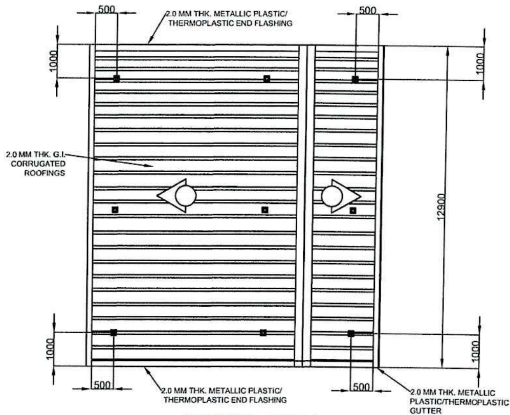
ROOFING DETAILS
